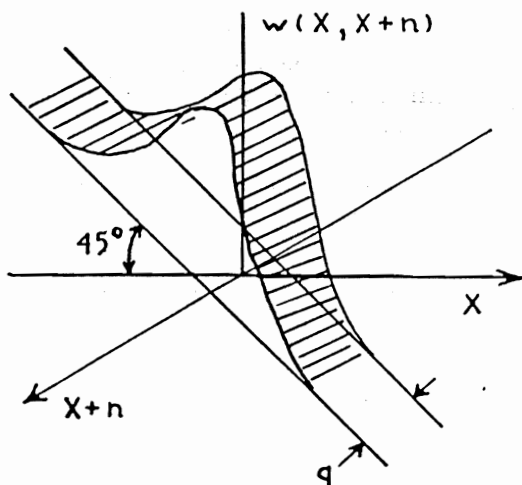
Fig. 12—Joint in-out distribution for a quantizer and for a source of additive independent quantization noise.
