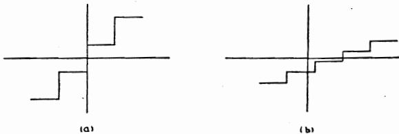
Fig. 2—More general quantizers.
