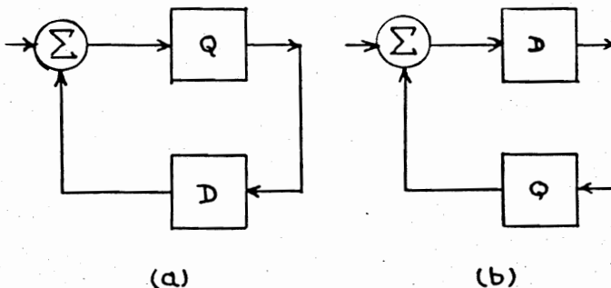
Fig. 18—Quantizer sample-data feedback systems.
