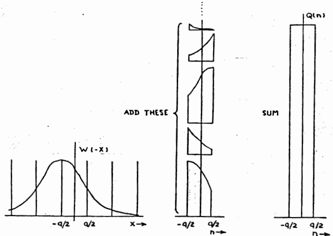
Fig. 9—Construction of distribution of quantization noise.
