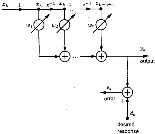
Fig. 2. Adaptive transversal digital filter.
