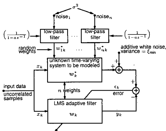
Fig. 8. Modeling an unknown time-varying system.
