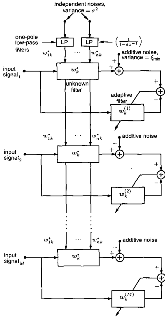
Fig. 9. An ensemble of nonstationary adaptive processes.
