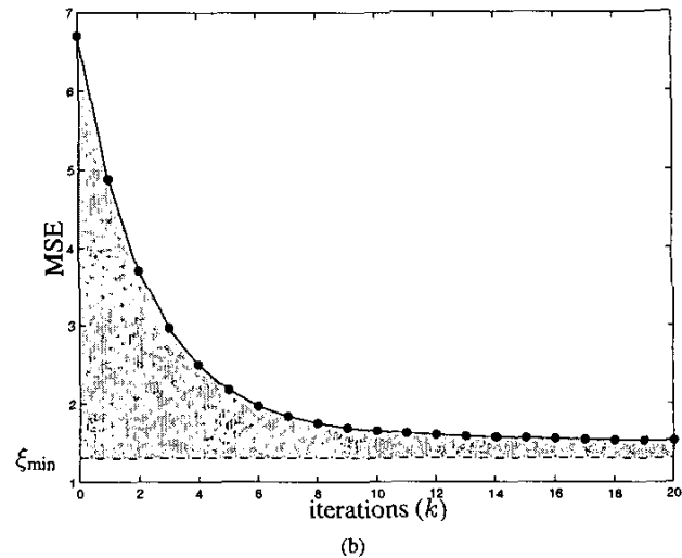
Fig. 7. Idealized learning curves (no gradient noise): (a) single-exponential, (b) two-exponential. The shaded area represents the excess error energy.
