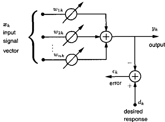
Fig. 1. Adaptive linear combiner.
