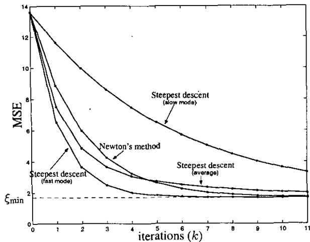
Fig. 6. Steepest descent and Newton's method learning curves.
