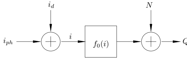
Figure 4. Sensor model after combining the noise sources.
