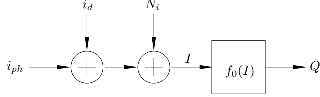
Figure 5. Sensor model with input referred noise.
