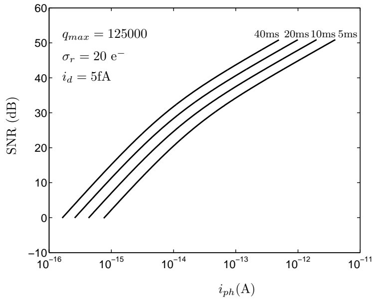
Figure 9. SNR vs. i_{ph} at four integration times.
