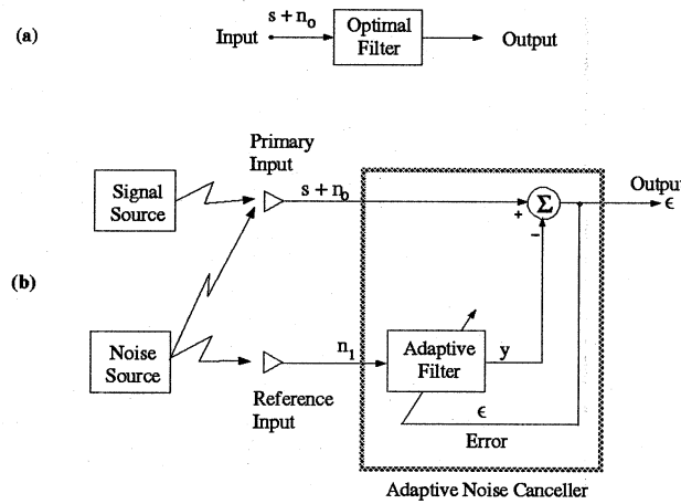
Figure 9: Separation of signal and noise: (a) classical approach; (b) adaptive noise cancelling approach.
