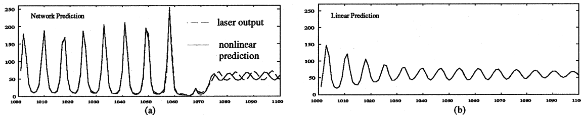
Figure 21: Time series predictions: (a) Closed loop neural network prediction does very well. (b) Iterated 25th order linear predictor does poorly.
