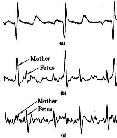
Figure 11: Result of fetal ECG experiment (bandwidth, 3-35 Hz; sampling rate, 256 Hz): (a) reference input (chest lead); (b) primary input (abdominal lead); (c) noise canceller output.
