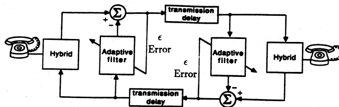
Figure 12: Long-distance system with adaptive echo cancellation.
