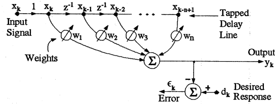
Figure 2: An adaptive linear filter.
