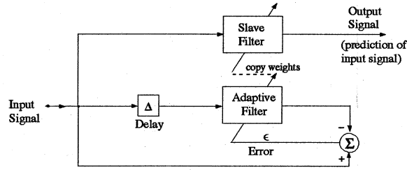
Figure 18: An adaptive linear statistical predictor.
