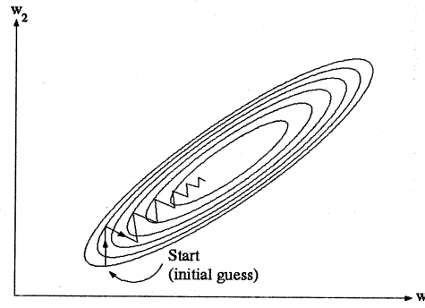
Figure 3: A quadratic MSE function explored by steepest descent.
