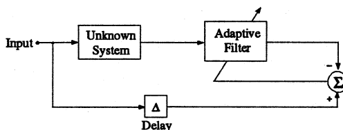
Figure 13: Inverse modeling.
