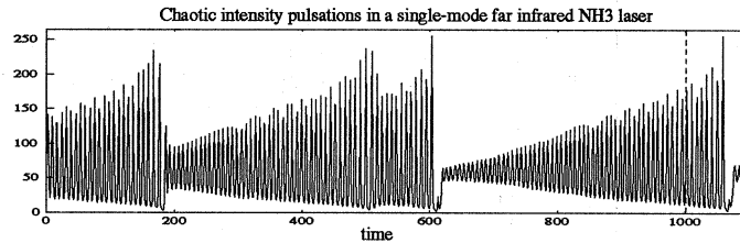
Figure 20: Chaotic light intensity pulsations on an NH_3 laser.
