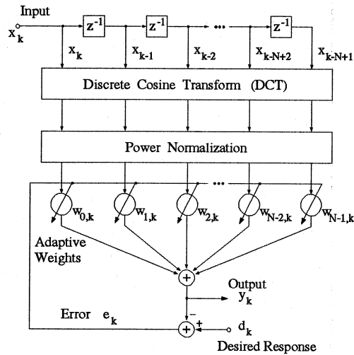
Figure 4: The DCT/LMS Adaptive Filter.
