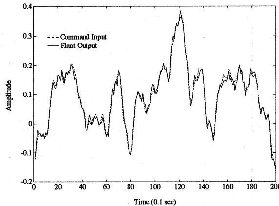
Figure 15: Tracking between command input and plant output.
