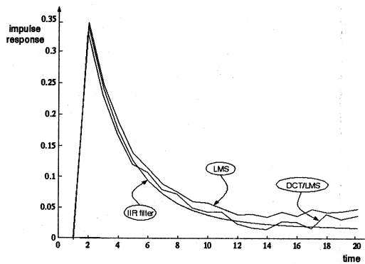
Figure 7: Impulse response of the plant, of the LMS filter, and of the DCT/LMS filter.
