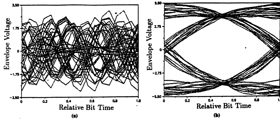
Figure 17: Eye patterns produced by overlaying cycles of the received waveform: (a) before equalization; (b) after equalization.
