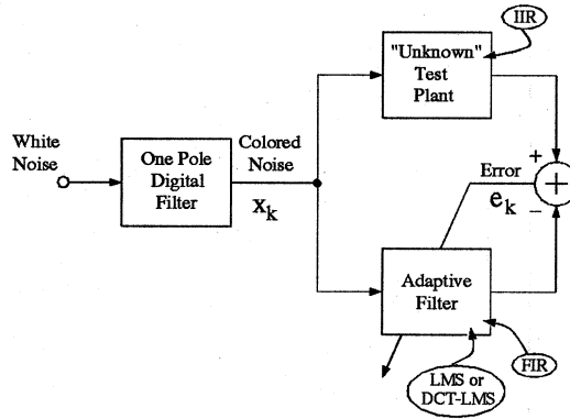
Figure 6: Using adaptive filters for plant modeling.
