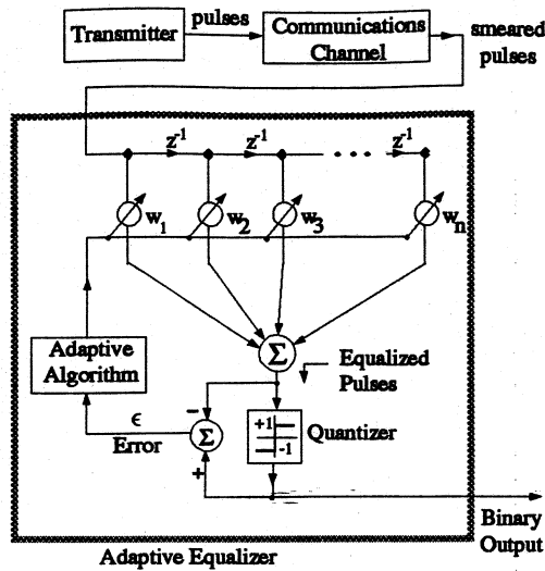
Figure 16: Adaptive channel equalizer with decision-directed learning
