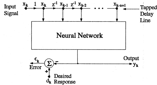
Figure 19: Adaptive nonlinear filter.
