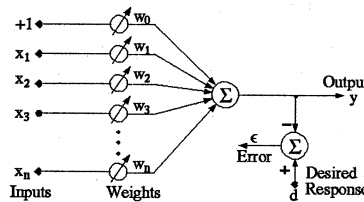
Figure 1: An adaptive linear combiner.
