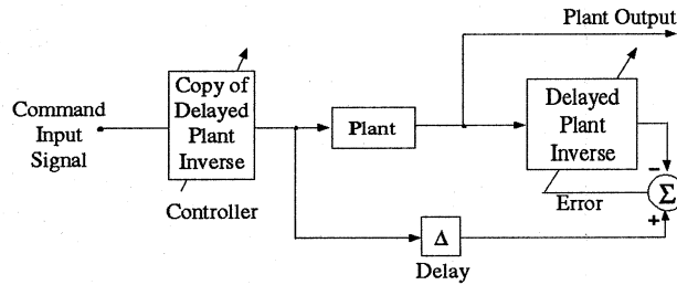
Figure 14: An adaptive inverse control system.
