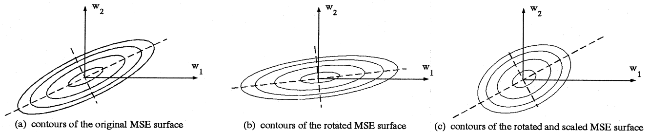
Figure 5: Rotation and scaling of MSE bowl by action of the DCT followed by power normalization.
