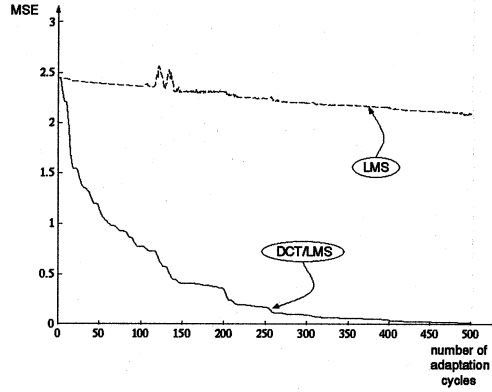
Figure 8: Learning curves for the LMS filter and the DCT/LMS filter.
