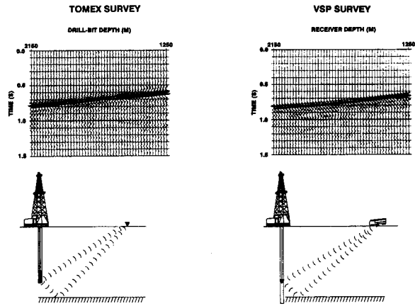
FIG. 5. Comparison between drill-bit source inverse VSP and conventional VSP full wave field data.
