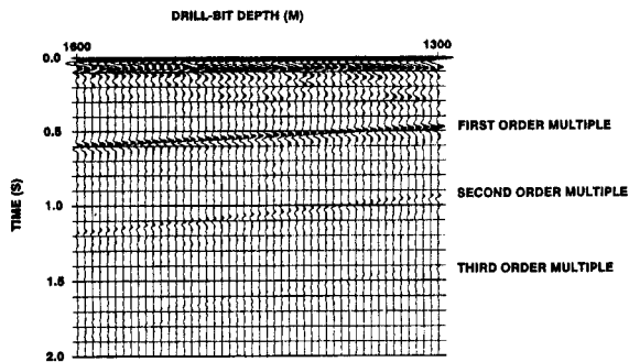
FIG. 4. Pilot-signal autocorrelations for drilling depths from 1300 to 1600 m. Depth spacing is 6 m.
