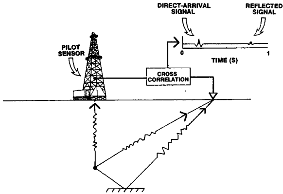
FIG. 2. Diagram showing how seismic energy propagates from drill bit to pilot sensor and to geophones.
