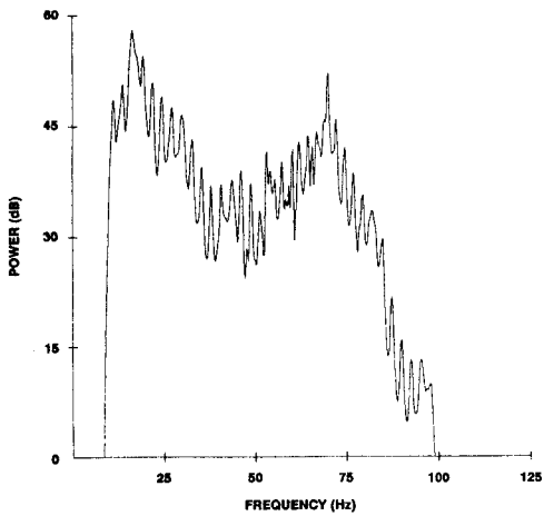
FIG. 3. Pilot-signal spectrum from a drilling depth of 900 m. Resonance peaks spaced at 2.5 Hz are due to drillpipe multiples.
